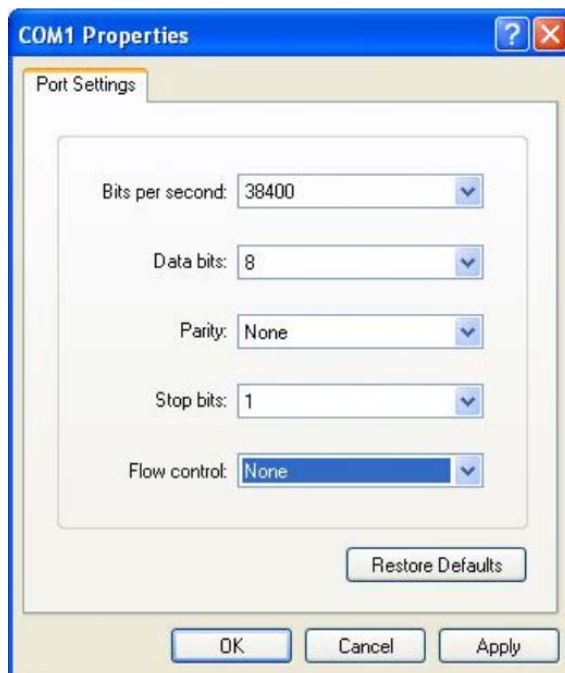
Figure C-5 Port Settings
