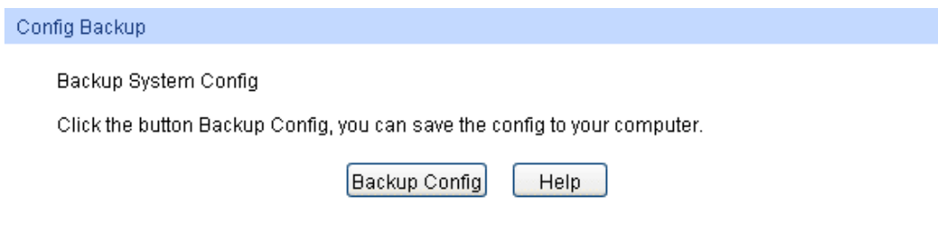
Figure 4-14 Config Backup
