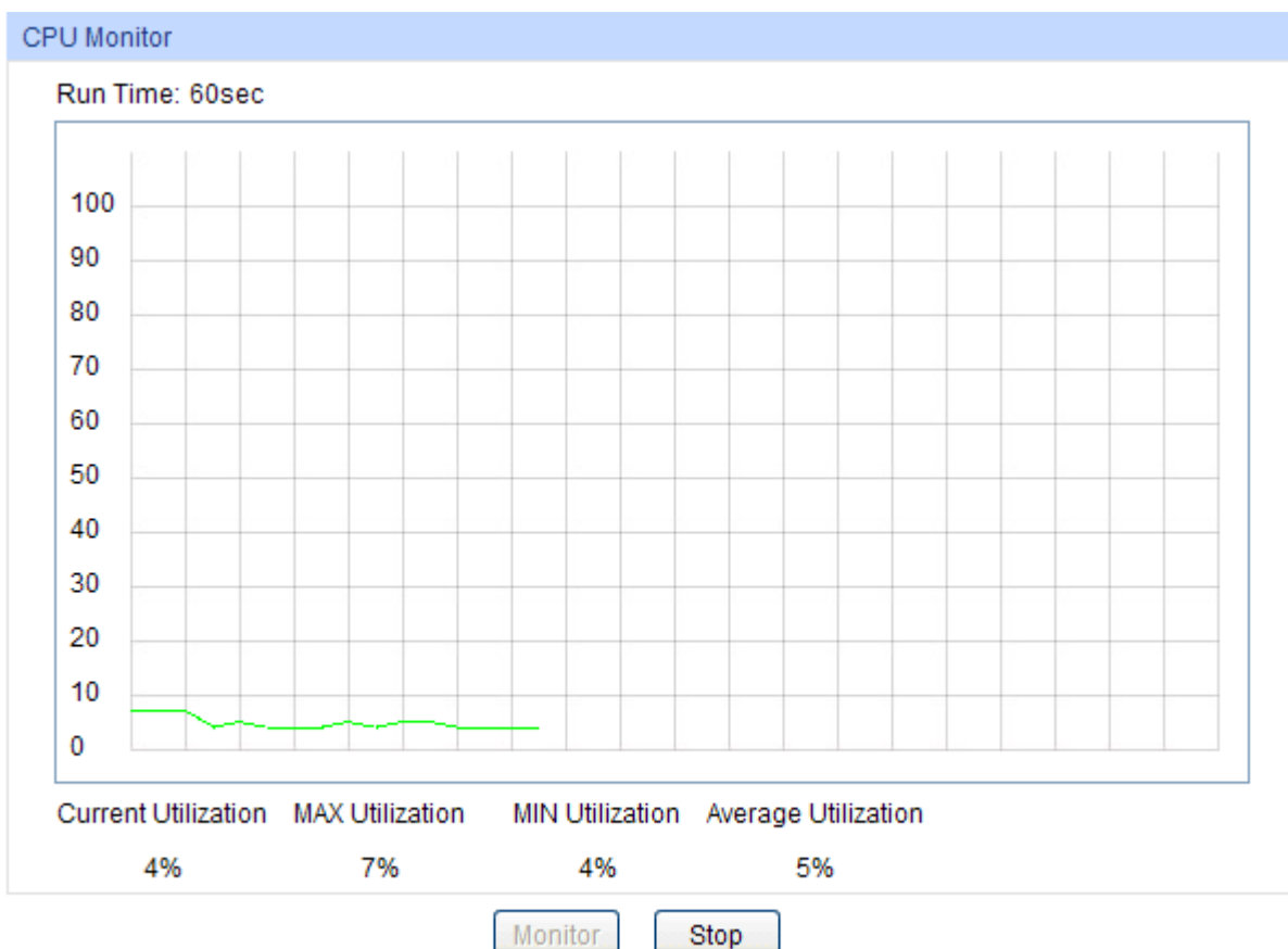
Figure 16-1 CPU Monitor
