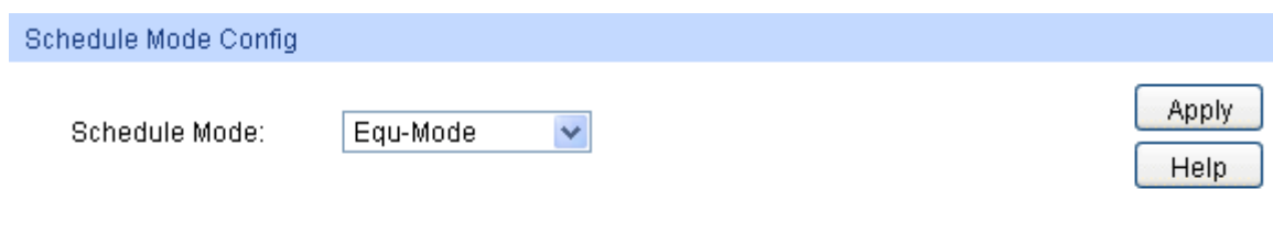
Figure 9-9 Schedule Mode
