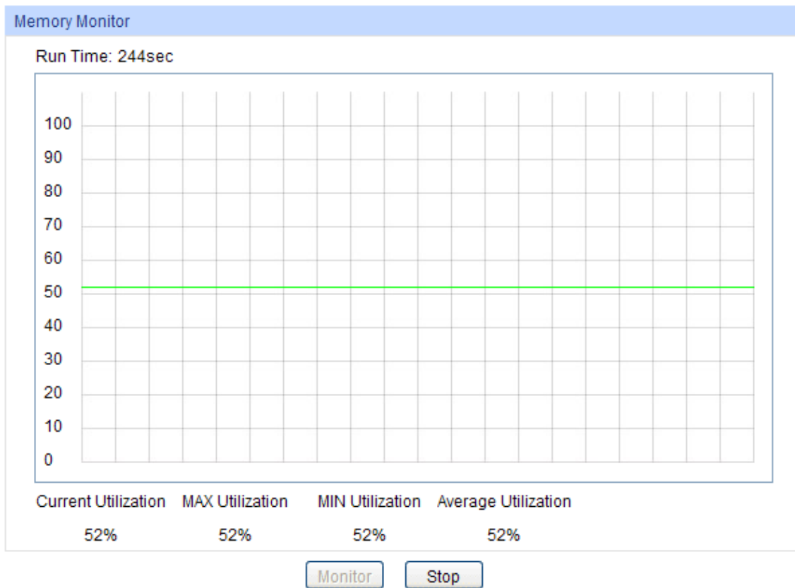
Figure 16-2 Memory Monitor
