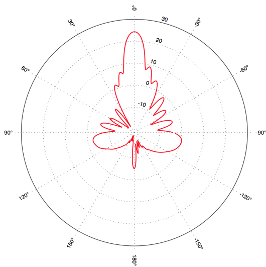
Horizontal 90 deg
