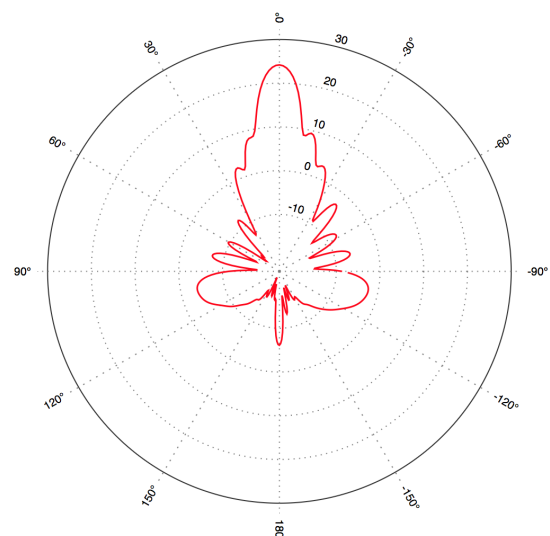
Vertical 0 deg
