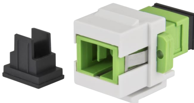
Adapter SC/APC-1SM-K
